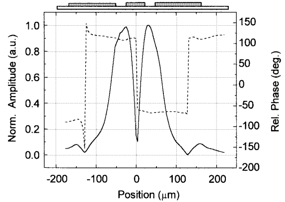
Fig. 3. Electrooptic mapping of tangential-field component in the x -direction of the even mode on a CPW (transverse direction) measured using LiTaO 3 , f = 15 \text{ GHz} , solid line: normalized amplitude, dashed line: phase.
