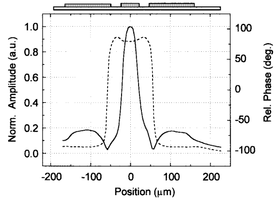
Fig. 2. Electrooptic mapping of the normal-field component of the even mode on a CPW (transverse direction) measured using BSO, f = 5 \text{ GHz} , solid line: normalized amplitude, dashed line: phase (the center conductor has a width of 40 \mu\text{m} , with spacings of 24 \mu\text{m} ).
